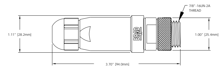
Male Straight w/ External Threads
